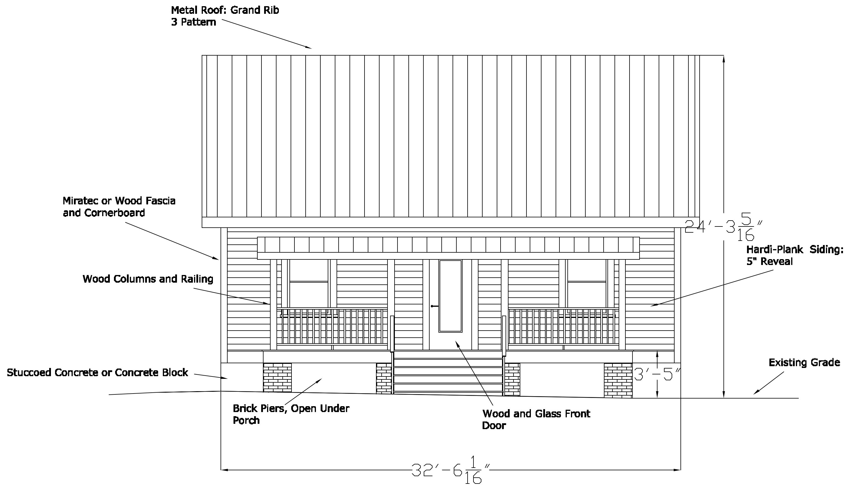
East / Front Elevation 345 Lyndon Avenue (Proposed)
